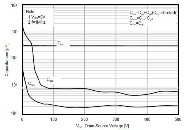
Figure10. Capacitance
