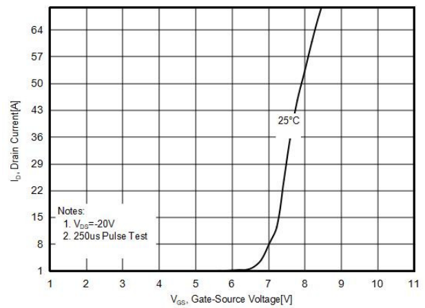
Figure10. Transfer characteristics
