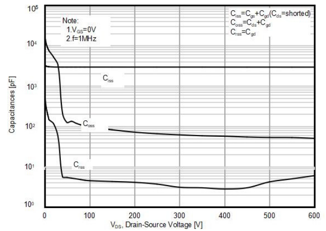
Figure2. Capacitance
