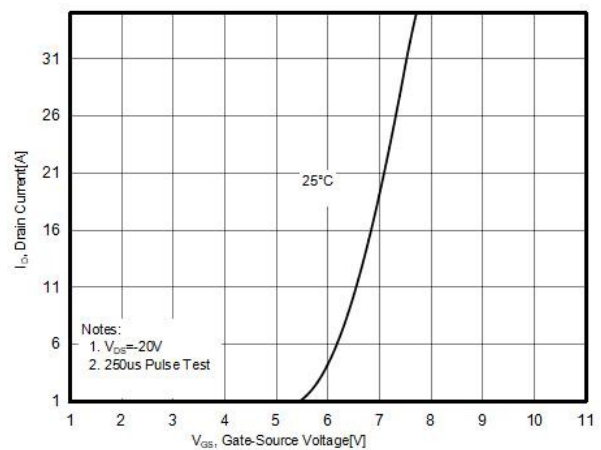
Figure6. Transfer characteristics
