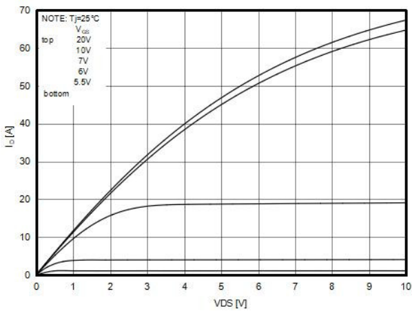
Figure9. Output characteristics
