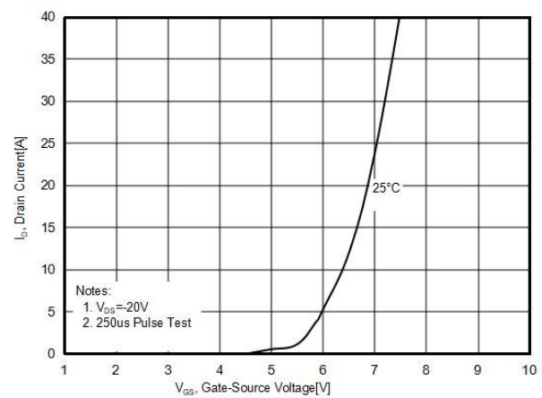
Figure6. Transfer characteristics
