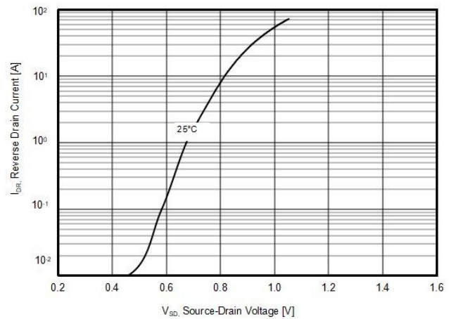
Figure4. Source-Drain Diode Forward Voltage
