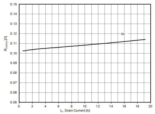
Figure8. Static drain-source on resistance
