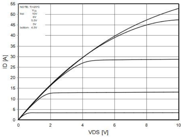
Figure7. Output characteristics
