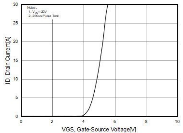
Figure6. Transfer characteristics
