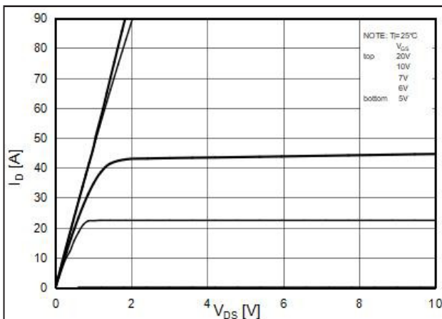
Figure3. Output characteristics
