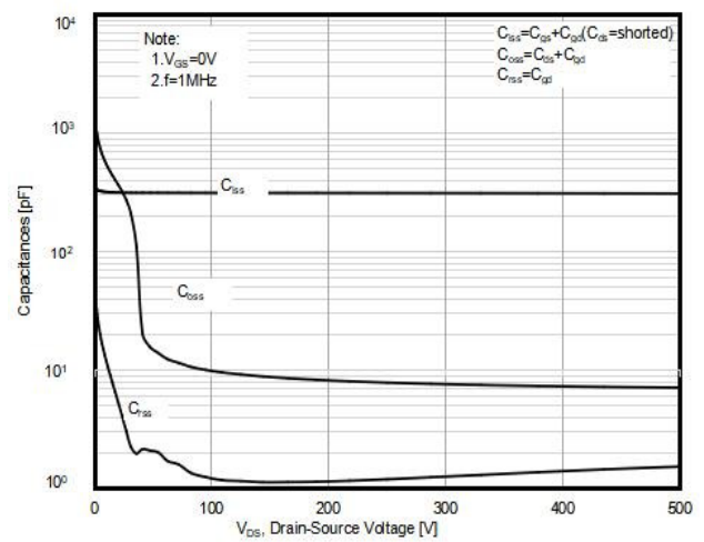
Figure10. Capacitance
