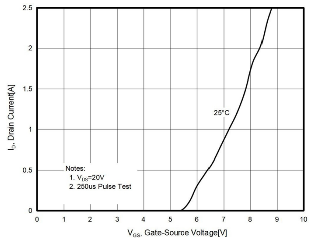
Figure4. Transfer characteristics
