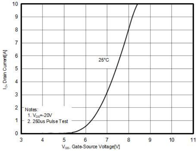
Figure1. Transfer characteristics
