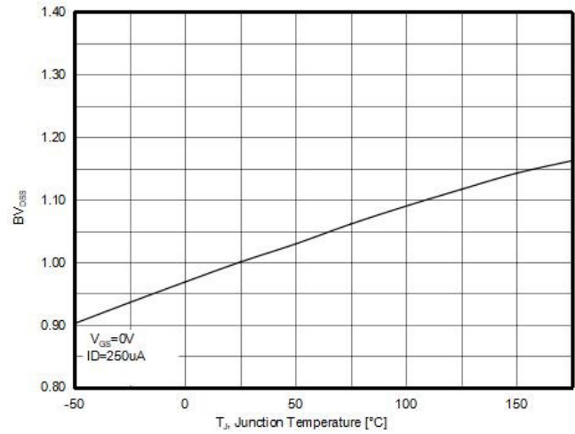
Figure4. BV_{DSS} vs Junction Temperature
