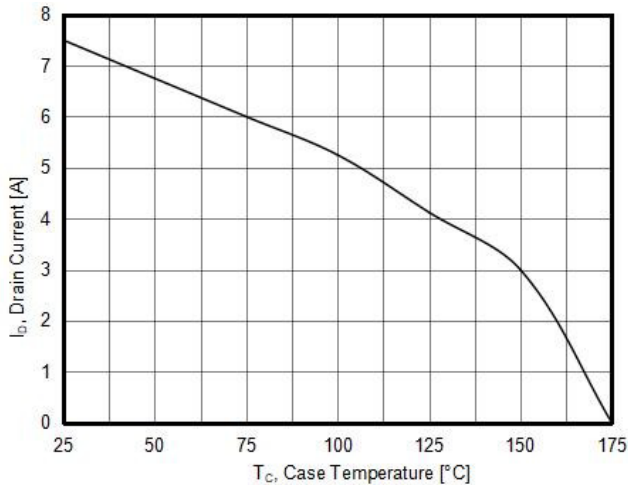
Figure5. Maximum I_D vs Junction Temperature
