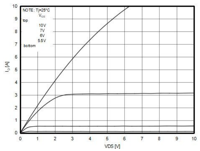
Figure2. Output characteristics
