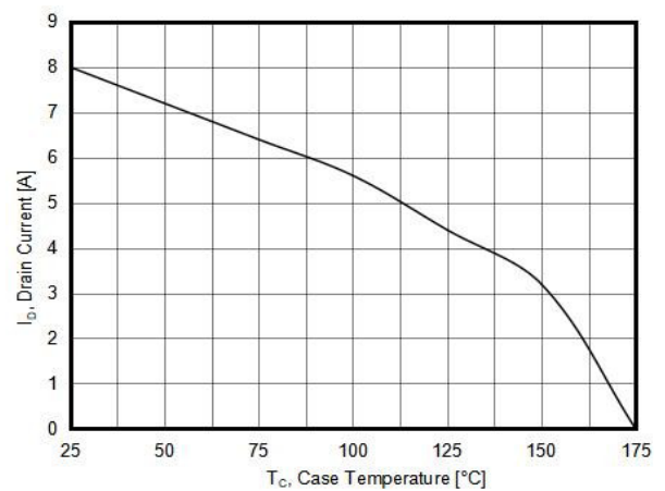
Figure6. Maximum I_D vs Junction Temperature
