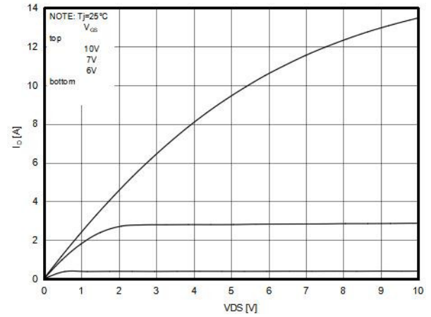
Figure8. Output characteristics
