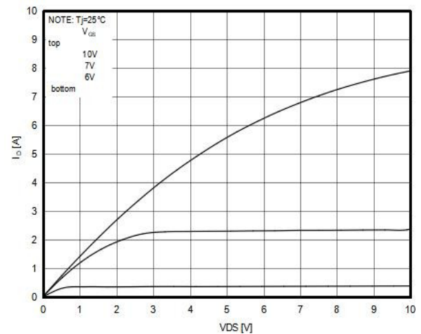
Figure6. Output characteristics
