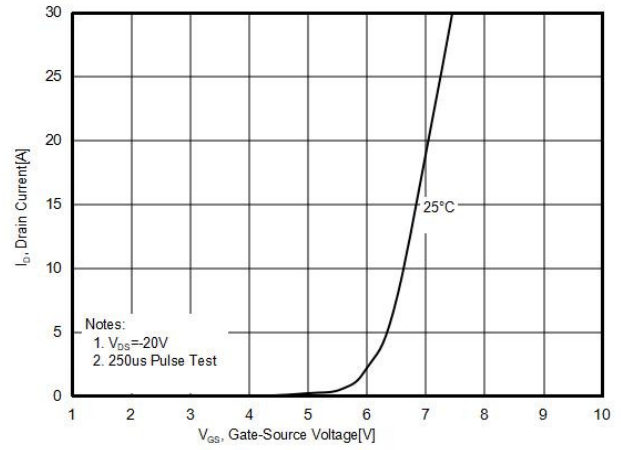
Figure10. Transfer characteristics
