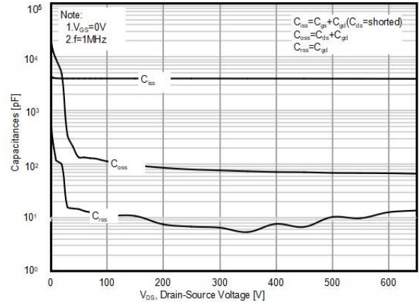
Figure2. Capacitance
