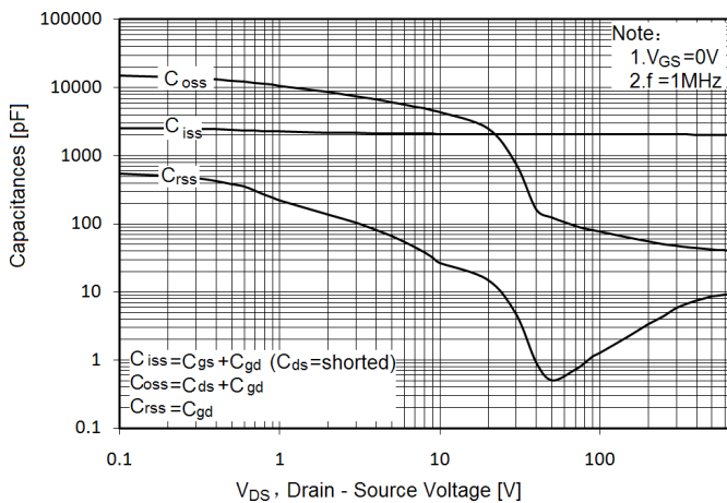
Figure11. Capacitance
