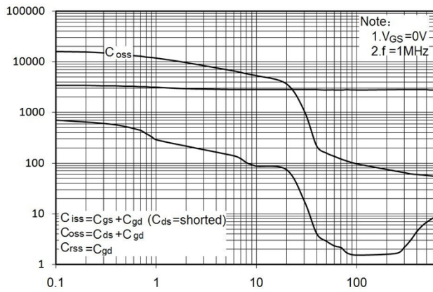
Figure9. Capacitance
