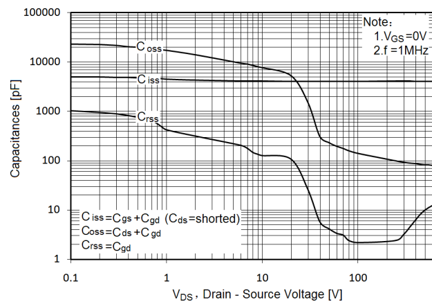
Figure11. Capacitance
