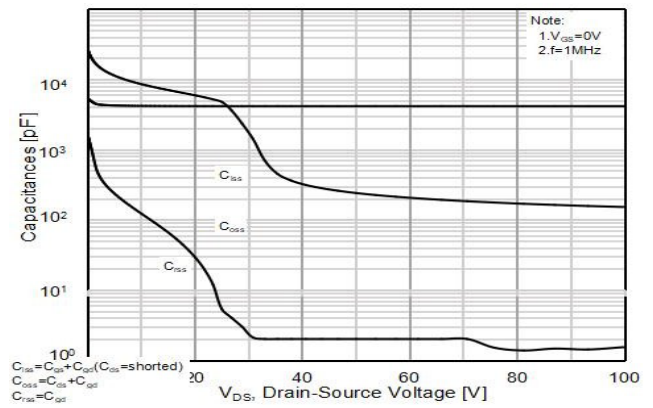
Figure2. Capacitance
