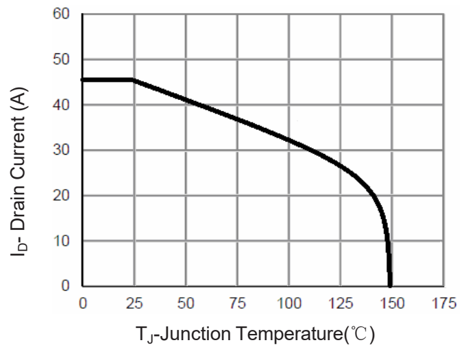
Figure 9 Current De-rating
