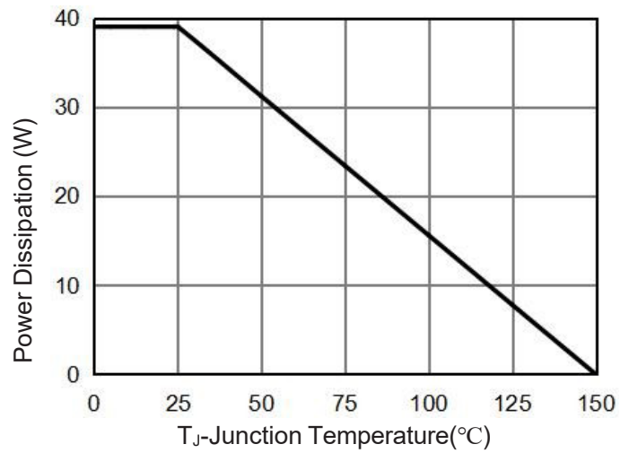
Figure 9 Power De-rating
