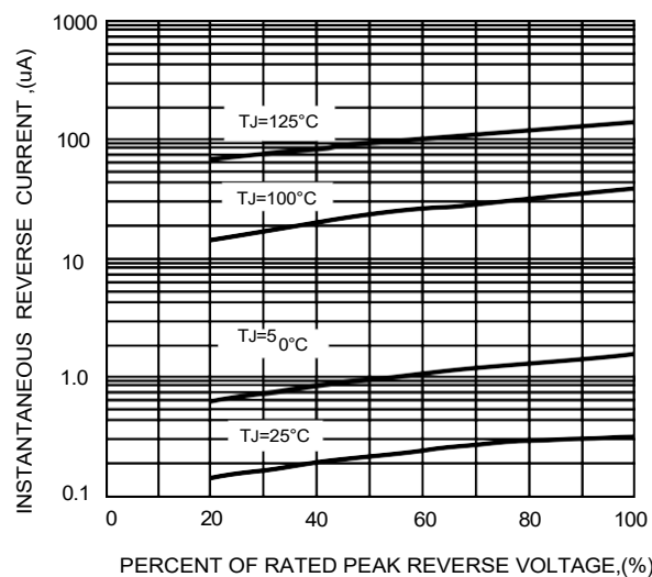
FIG.5-TYPICAL REVERSE CHARACTERISTICS
