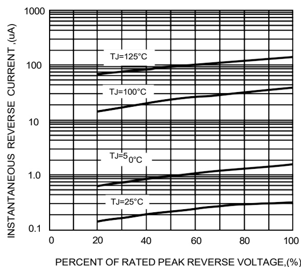
FIG.5-TYPICAL REVERSE CHARACTERISTICS
