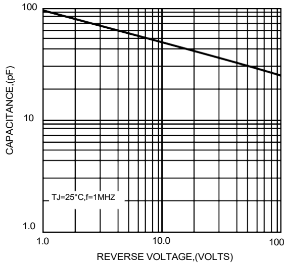
FIG.3-TYPICAL JUNCTION CAPACITANCE
