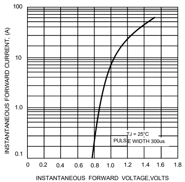
FIG.4-TYPICAL FORWARD CHARACTERISTICS
