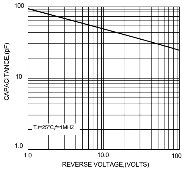
FIG.3-TYPICAL JUNCTION CAPACITANCE
