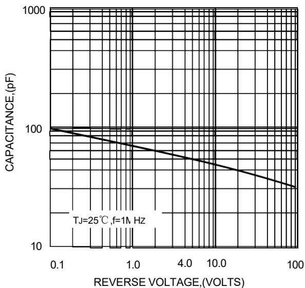
FIG.3-TYPICAL JUNCTION CAPACITANCE
