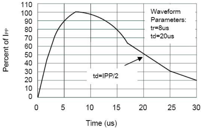
Pulse Waveform
