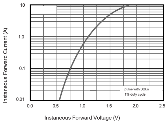
Fig.3 Typical Instaneous Forward Characteristics T_J = 25^\circ C
