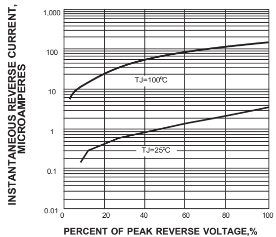
FIG. 4-TYPICAL REVERSE CHARACTERISTICS
