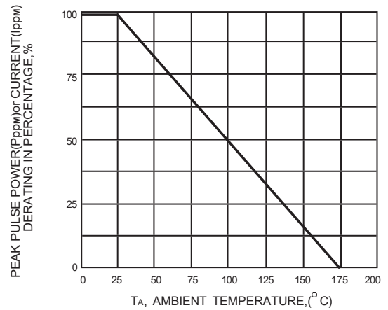
FIG. 2-PULSE DERATING CURVE
