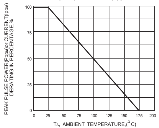
FIG. 2-PULSE DERATING CURVE
