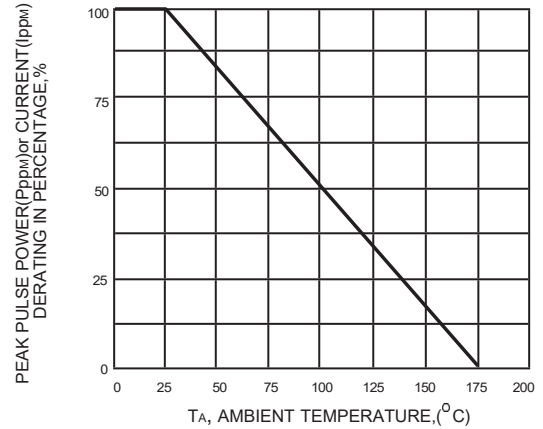
FIG. 2-PULSE DERATING CURVE
