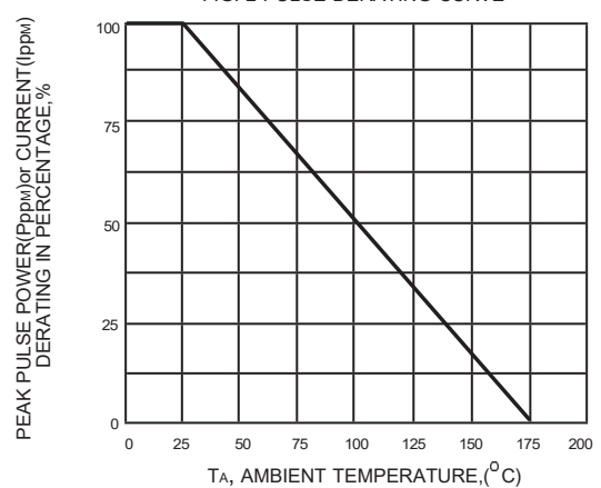
FIG. 2-PULSE DERATING CURVE
