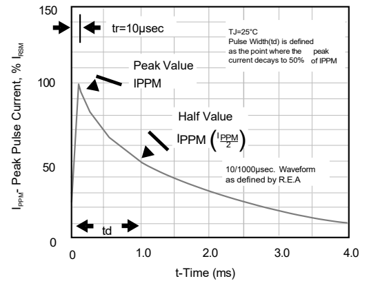
Figure 4 - Pulse Waveform
