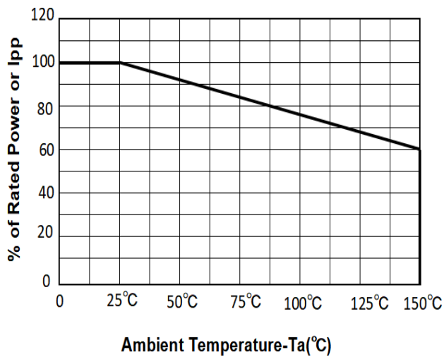
Fig.3 Power Derating
