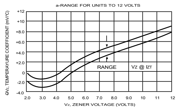
FIG.7- TEMPERATURE COEFFICIENTS
