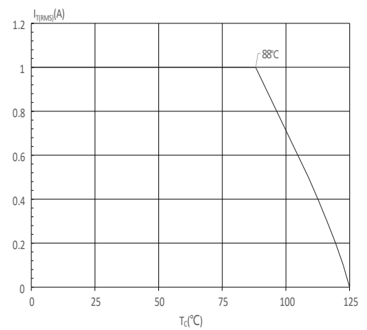
FIG : RMS on-state current versus case temperature
