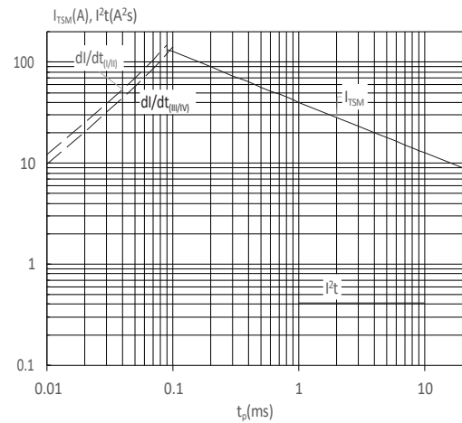
FIG : Non-repetitive surge peak on-state current for a sinusoidal pulse with width t_p < 20\text{ms} , and corresponding value of I^2t ( I - II : dl/dt < 50\text{A}/\mu\text{s} ; III-IV : dl/dt < 30\text{A}/\mu\text{s} )
