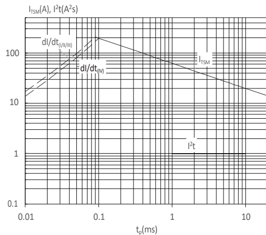
FIG : Non-repetitive surge peak on-state current for a sinusoidal pulse with width t_p < 20\text{ms} , and corresponding value of I^2t ( I - II -III: di/dt < 50\text{A}/\mu\text{s} ; IV: di/dt < 30\text{A}/\mu\text{s} )
