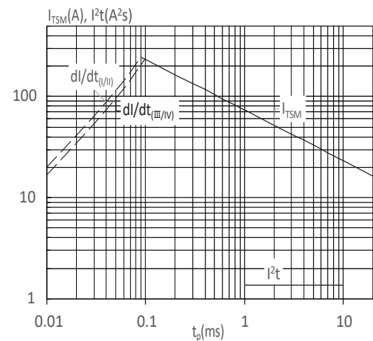
FIG : Non-repetitive surge peak on-state current for a sinusoidal pulse with width t_p < 20ms , and corresponding value of I^2t (I - II: dl/dt < 30A/\mu s ; III-IV: dl/dt < 20A/\mu s )
