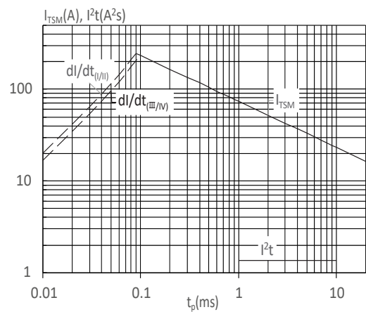
FIG : Non-repetitive surge peak on-state current for a sinusoidal pulse with width t_p < 20ms , and corresponding value of I^2t (I - II : di/dt < 30A/\mu s ; III-IV : di/dt < 20A/\mu s )
