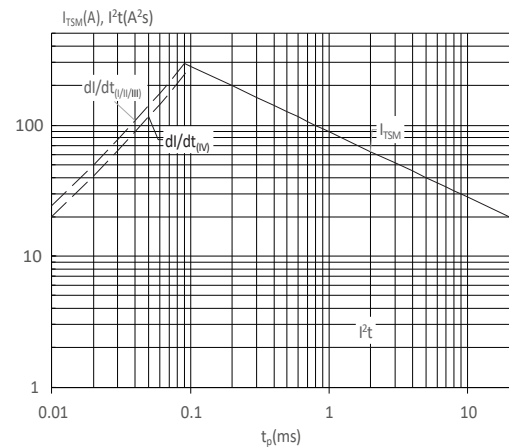
FIG : Non-repetitive surge peak on-state current for a sinusoidal pulse with width t_p < 20ms , and corresponding value of I^2t (I - II - III: dl/dt < 50A/\mu s ; IV: dl/dt < 30A/\mu s )
