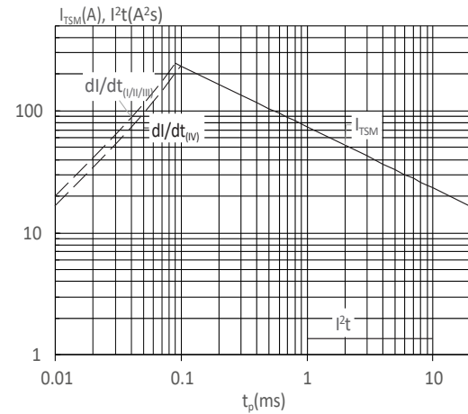
FIG : Non-repetitive surge peak on-state current for a sinusoidal pulse with width t_p < 20ms , and corresponding value of I^2t (I - II - III: di/dt < 50A/\mu s ; IV: di/dt < 30A/\mu s )
