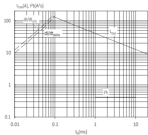
FIG : Non-repetitive surge peak on-state current for a sinusoidal pulse with width t_p < 20\text{ms} , and corresponding value of I^2t (I - II : di/dt < 50\text{A}/\mu\text{s} ; III-IV : di/dt < 30\text{A}/\mu\text{s} )
