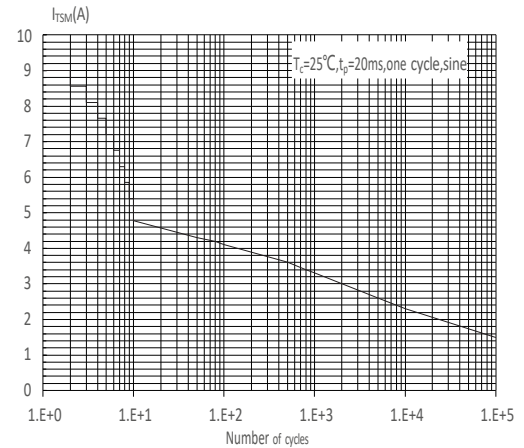
FIG : Non-repetitive surge peak on-state current for a sinusoidal pulse with width t_p < 20\text{ms} , and corresponding value of I^2t (I - II : di/dt < 50\text{A}/\mu\text{s} ; III-IV : di/dt < 30\text{A}/\mu\text{s} )
