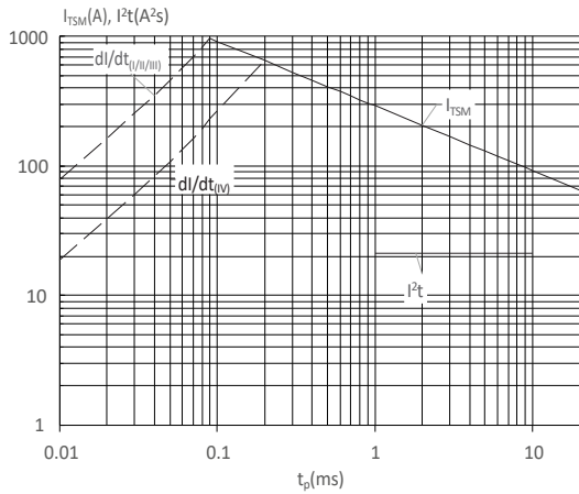
FIG : Non-repetitive surge peak on-state current for a sinusoidal pulse with width t_p < 20\text{ms} , and corresponding value of I^2t ( I - II -III: di/dt < 80\text{A}/\mu\text{s} ; IV: di/dt < 40\text{A}/\mu\text{s} )
