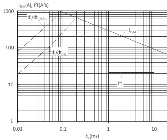
FIG : Non-repetitive surge peak on-state current for a sinusoidal pulse with width t_p < 20ms , and corresponding value of I^2t ( I - II -III: dl/dt < 100A/\mu s ; IV: dl/dt < 50A/\mu s )
