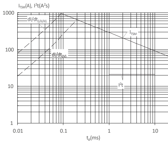
FIG : Non-repetitive surge peak on-state current for a sinusoidal pulse with width t_p < 20\text{ms} , and corresponding value of I^2t ( I - II -III: di/dt < 100\text{A}/\mu\text{s} ; IV: di/dt < 50\text{A}/\mu\text{s} )
