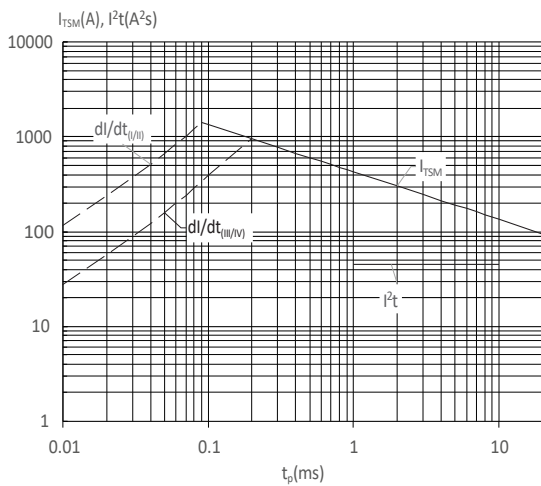
FIG : Non-repetitive surge peak on-state current for a sinusoidal pulse with width t_p < 20\text{ms} , and corresponding value of I^2t ( I - II : di/dt < 100\text{A}/\mu\text{s} ; III-IV : di/dt < 70\text{A}/\mu\text{s} )
