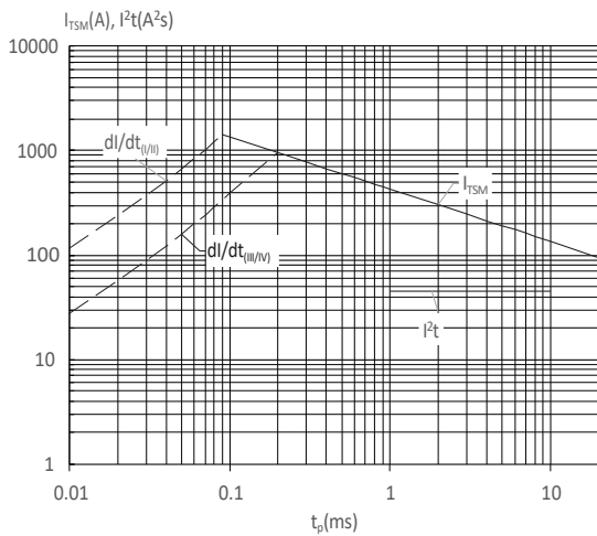
FIG : Non-repetitive surge peak on-state current for a sinusoidal pulse with width t_p < 20\text{ms} , and corresponding value of I^2t ( I_{II} : di/dt < 80\text{A}/\mu\text{s} ; III-IV : di/dt < 50\text{A}/\mu\text{s} )
