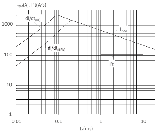
FIG : Non-repetitive surge peak on-state current for a sinusoidal pulse with width t_p < 20\text{ms} , and corresponding value of I^2t (I - II: di/dt < 80\text{A}/\mu\text{s} ; III-IV: di/dt < 50\text{A}/\mu\text{s} )
