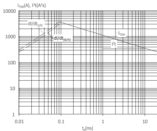
FIG : Non-repetitive surge peak on-state current for a sinusoidal pulse with width t_p < 20ms , and corresponding value of I^2t (I - II: di/dt < 80A/\mu s ; III-IV: di/dt < 40A/\mu s )
