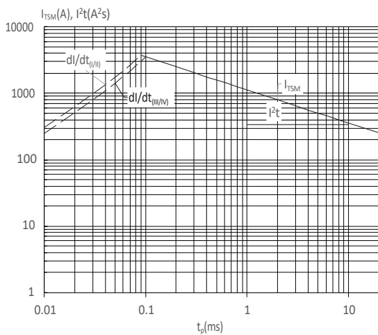
FIG : Non-repetitive surge peak on-state current for a sinusoidal pulse with width t_p < 20\text{ms} , and corresponding value of I^2t (I - II: di/dt < 80\text{A}/\mu\text{s} ; III-IV: di/dt < 40\text{A}/\mu\text{s} )
