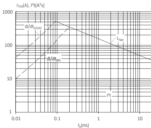
FIG : Non-repetitive surge peak on-state current for a sinusoidal pulse with width t_p < 20ms , and corresponding value of I^2t (I - II - III: di/dt < 80A/\mu s ; IV: di/dt < 40A/\mu s )
