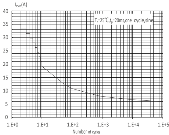
FIG : Non-repetitive surge peak on-state current for a sinusoidal pulse with width t_p < 20ms , and corresponding value of I^2t (I - II - III: di/dt < 80A/\mu s ; IV: di/dt < 40A/\mu s )
