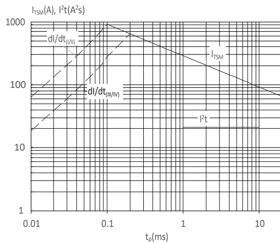
FIG : Non-repetitive surge peak on-state current for a sinusoidal pulse with width t_p < 20ms , and corresponding value of I^2t ( I - II : di/dt < 100A/\mu s ; III-IV : di/dt < 50A/\mu s )
